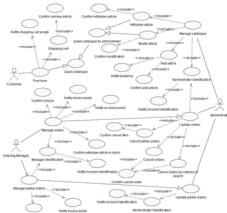
Figure 1. The Internet Shopping use case diagram
