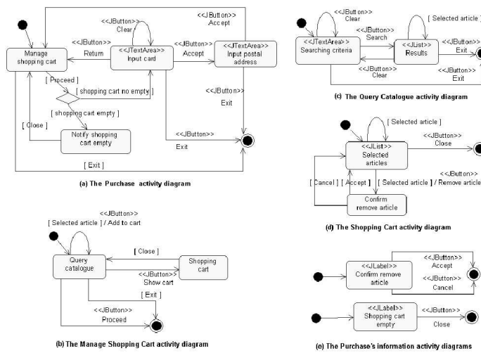
Figure 2. The whole activity diagram of the Purchase use case
